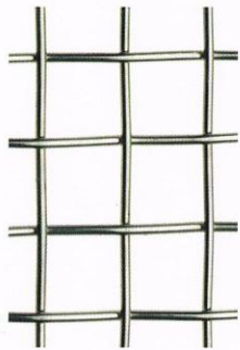
Apt 11.2 Dia 1.6
