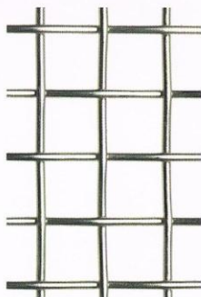
Apt 10 Dia 2.0
