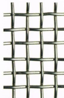
Apt 6.3 Dia 2.0
