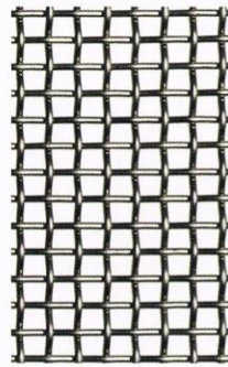
Apt 3.15 Dia 1.2
